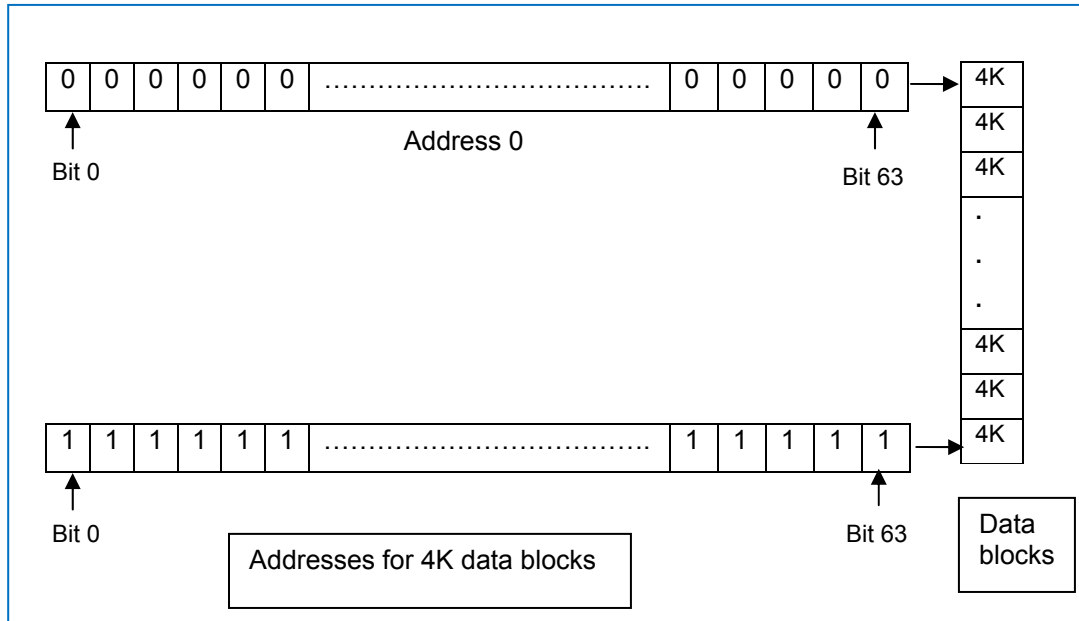
Figure 4) 64-bit addressing makes it feasible to increase the aggregate size.
