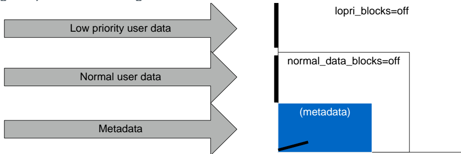
Figure 6) Metadata caching.
