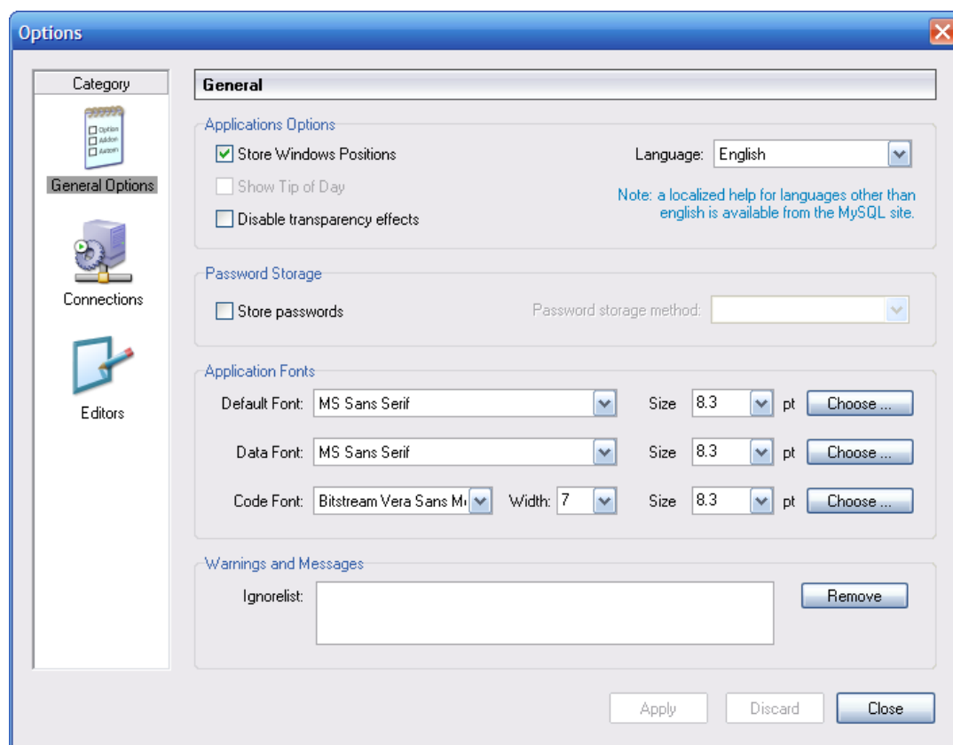
Figure 9.1. Options dialog
