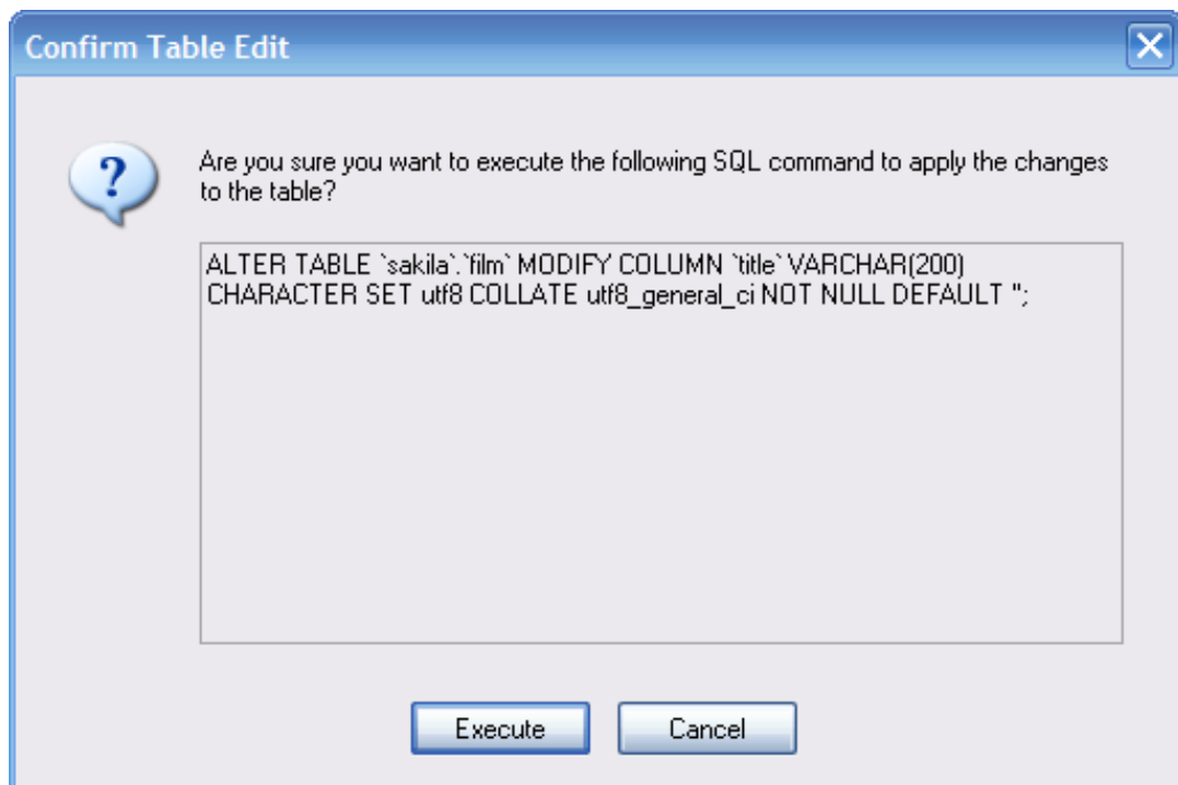
Figure 8.4. The Confirm Table Edit dialog
