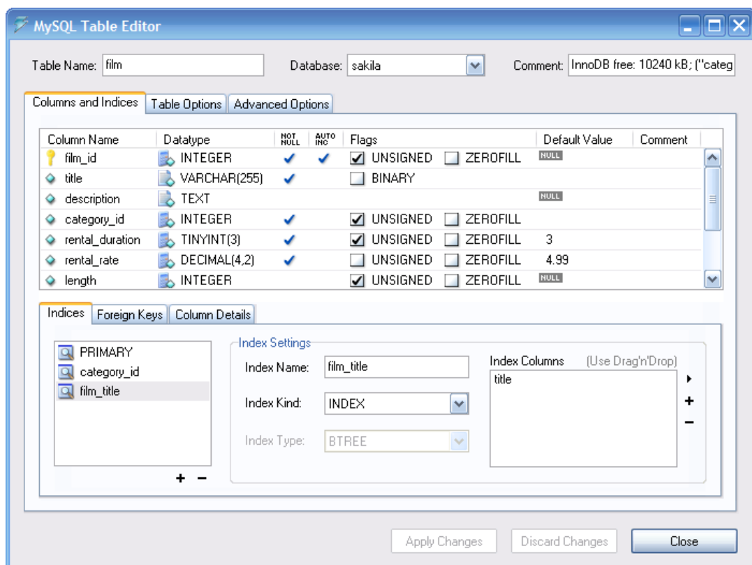
Figure 8.1. The MySQL Table Editor
